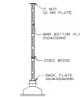
ISMC COLUMN
