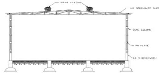
SECTION X-X' SCALE 1:100
