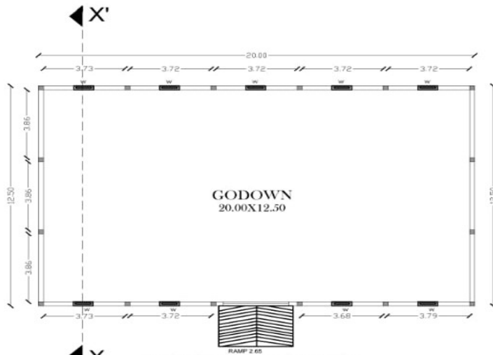
PROPOSED GODOWN PLAN SCALE 1:100
